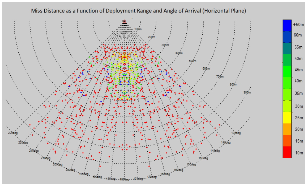
Figure 11 Miss Distance Horizontal Plane - No Maneuver
