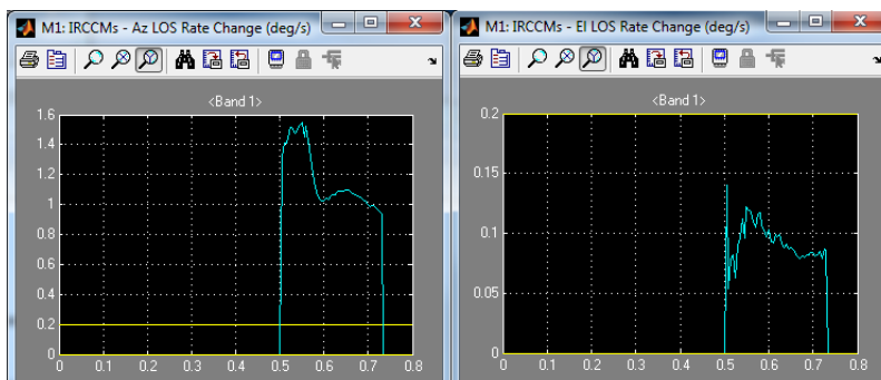
Figure 7 LOS Rate Change IRCCM Scores
