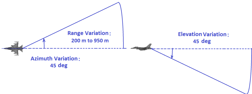
Figure 9 Engagement Geometry Variation
