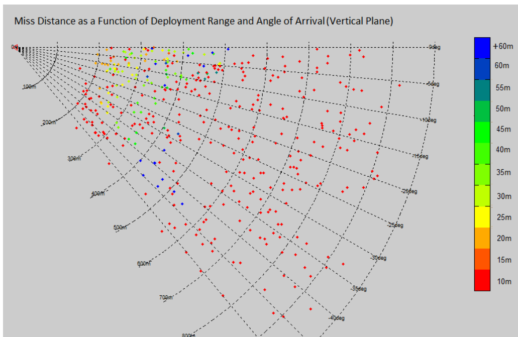
Figure 12 Miss Distance Vertical Plan - No Maneuver
