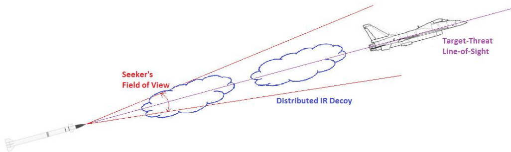
Figure 8 Ideal Engagement Geometry
