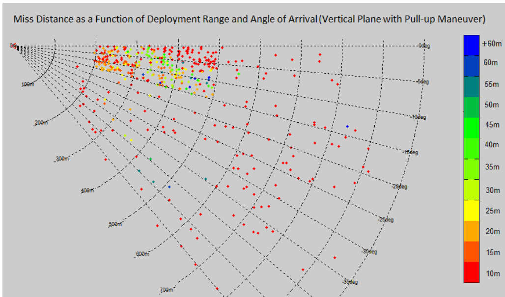
Figure 14 Miss Distance Vertical Plan - With Pull-up Maneuver
