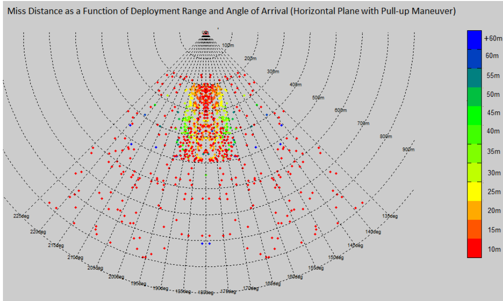
Figure 13 Miss Distance Horizontal Plane - With Pull-up Maneuver
